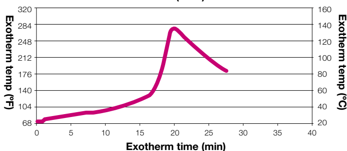
Typical Exotherm Curve for MA310 (10g mass) at 74°F (23°C) 5
