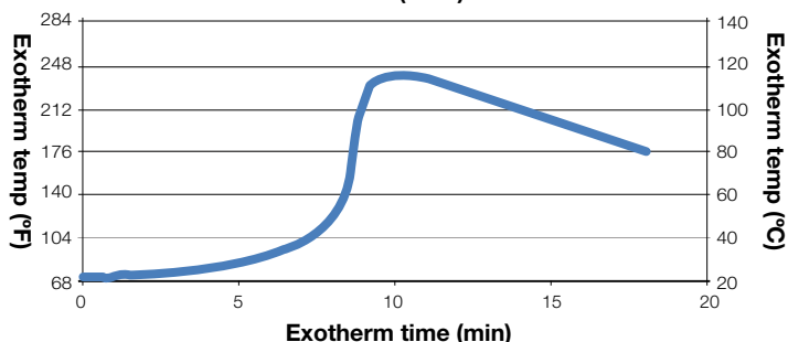
Typical Exotherm Curve for MA1020 (10g mass) at 74°F (23°C) 5
